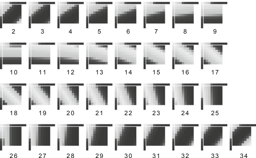
Angular modes
